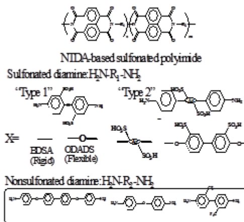
Fig.1 Chemical structures of sulfonated polyimides
